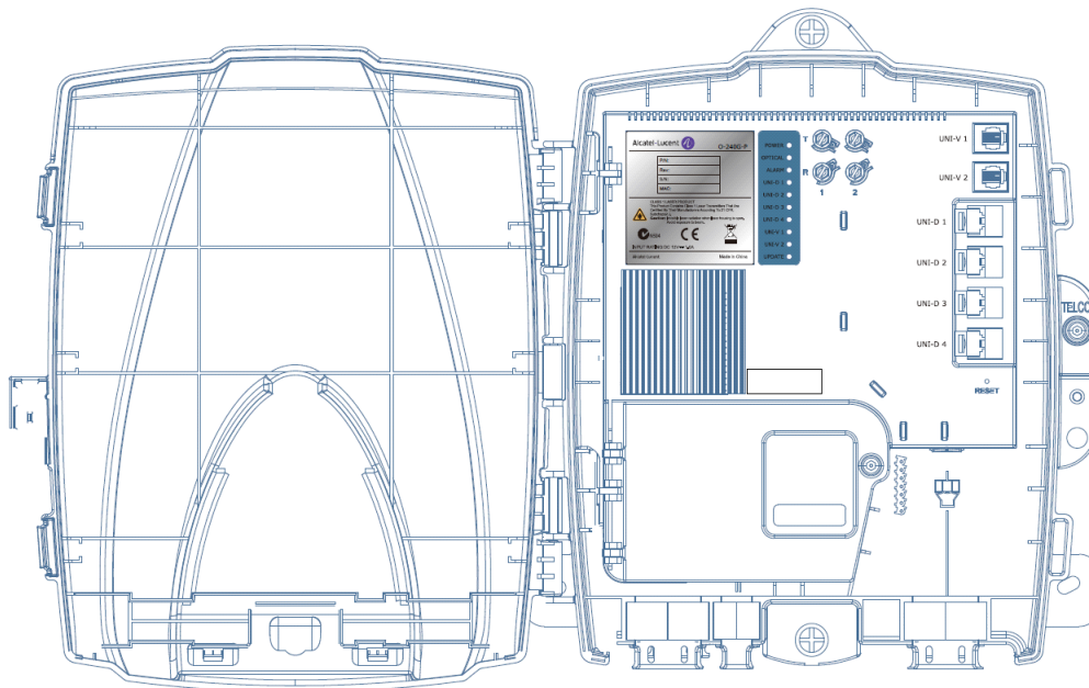
Figure 33 Outdoor NTU-R
